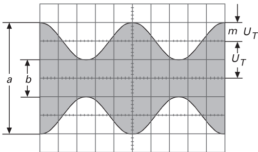
Figure 2 Amplitude modulated oscillator: F = 1 \text{ MHz} ; f = 1 \text{ kHz} ; m = 50\% ; U_T = 28.3 \text{ mVrms} . If the two values a and b are read from the screen, the modulation factor is calculated from
